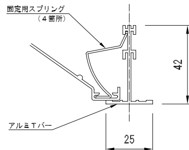
A部詳細 (S=1/2)
